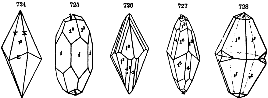
ANGLES OF SCALENOHEDRONS
